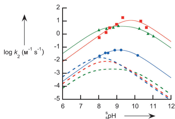
Figure 3. pH rate profile for the cleavage of BNPP catalyzed by 2 (green triangles), by 3 (red squares), and by 4' (blue circles) at 25 °C in anhydrous methanol, [buffer] = 0.05 M. Solid lines are from fitting Equation (1) to the data, [13] and the dashed lines illustrate the corresponding reactivity in water.
