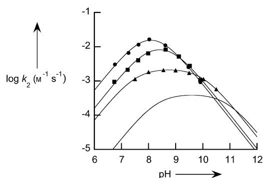
Figure 1. pH rate profile for the cleavage of BNPP catalyzed by 1 (no symbols; from reference [12]), by 2 (triangles), by 3 (squares), and by 4 (circles) at 25 °C ([buffer] = 0.05 M). Solid lines are from fitting Equation (1) to the data.
