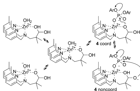
Scheme 2. Mechanistic scheme for reaction of 4 with BNPP.
